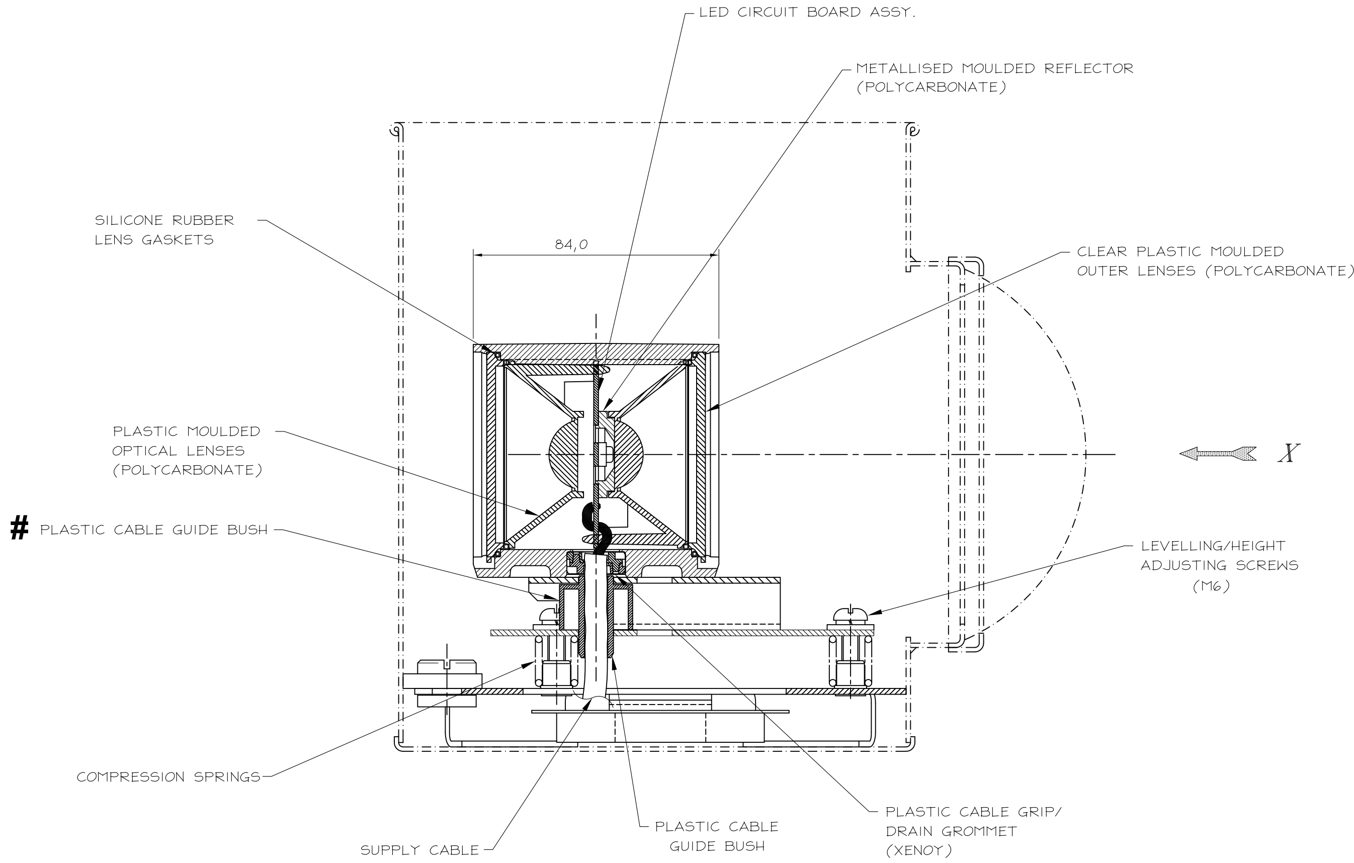
COMPOSITE SECTION
