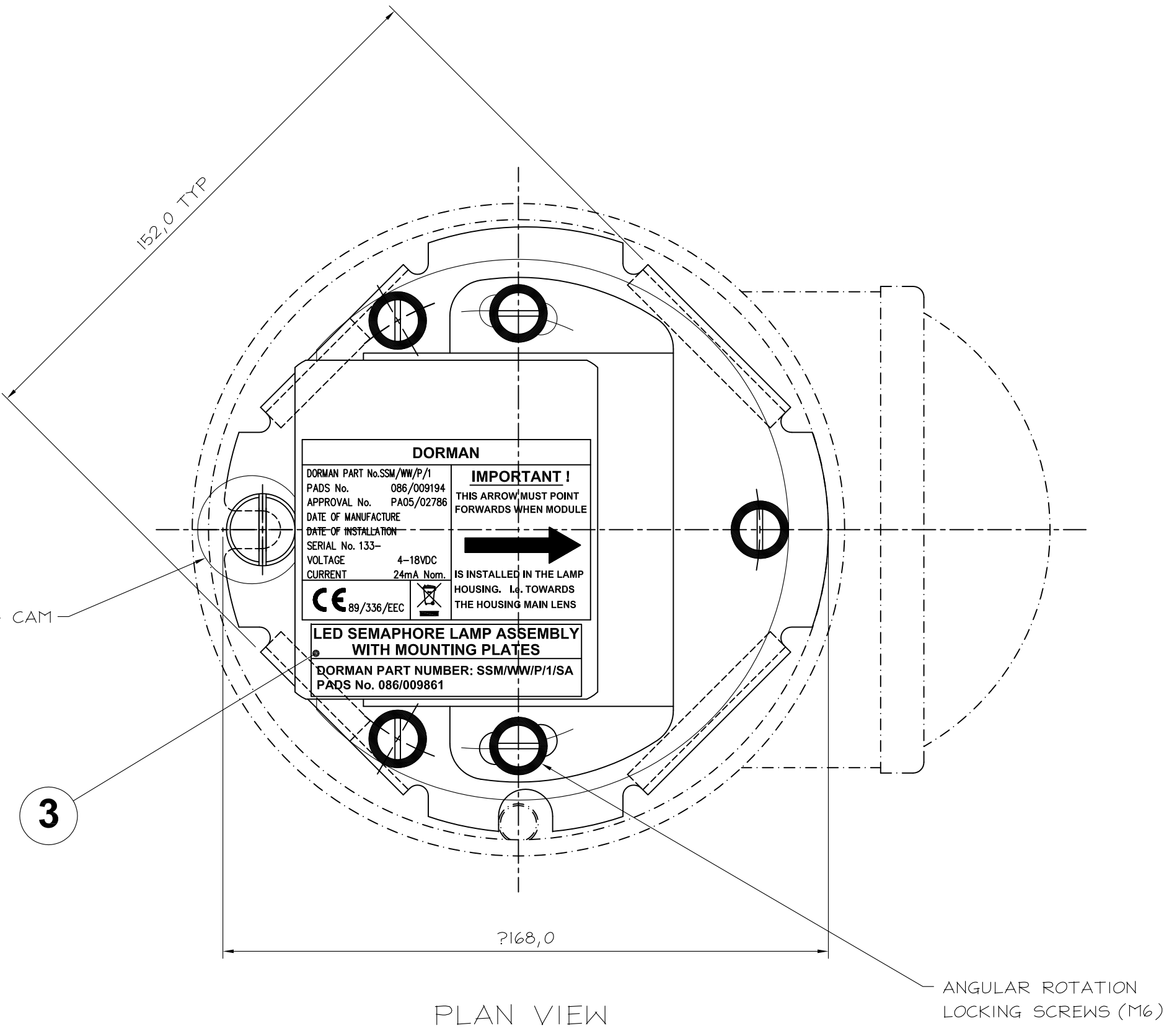
PLAN VIEW
