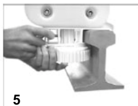
5 Pull release catch to remove.
