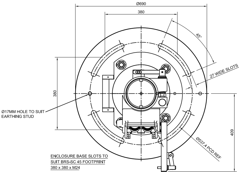
TRUNNION LOWERED THROUGH 90°
