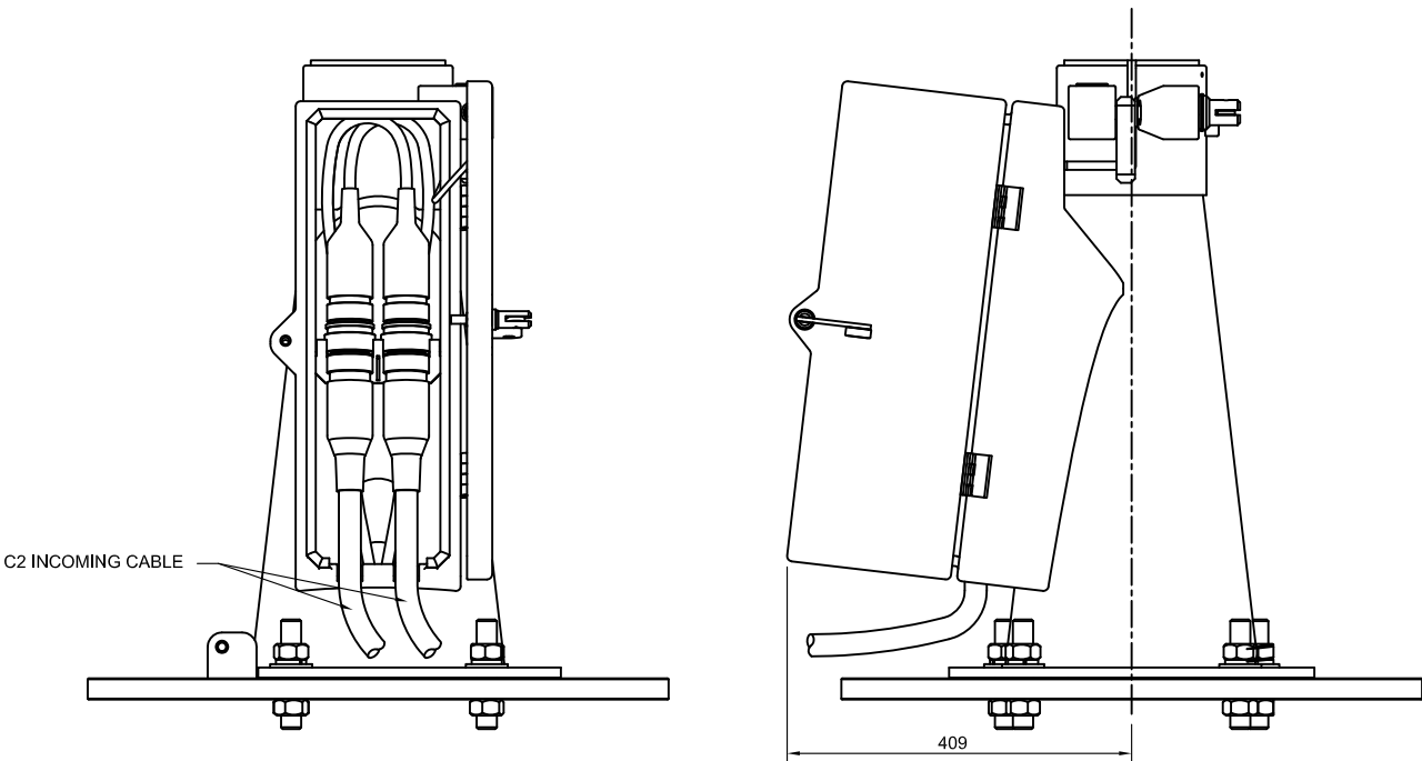
VIEWS WITH DOOR OPEN SHOWING INCOMING CABLE AND CONNECTORS
