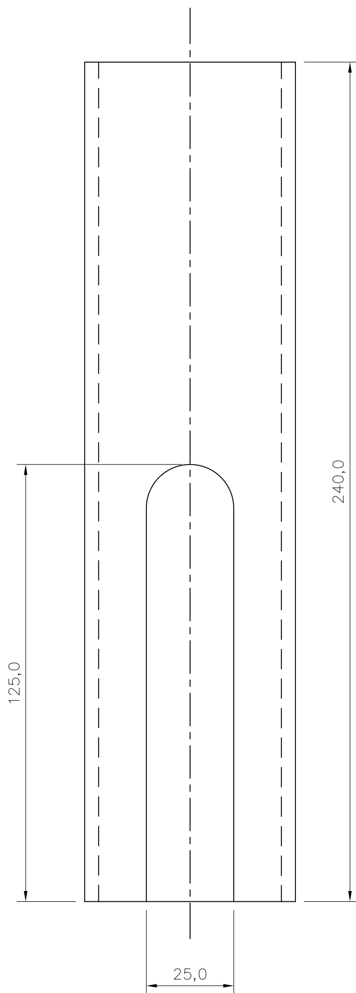
PART B – MOUNTING POST MATL: 60.3 O/D x 5.0 THICK CHS
