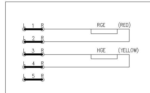
Signal connection arrangement
