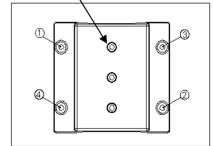
Clamp tightening sequence
