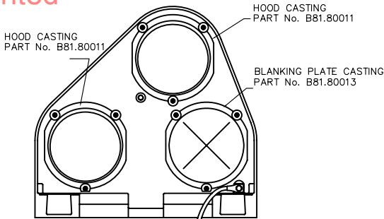
PL1W VERSION
