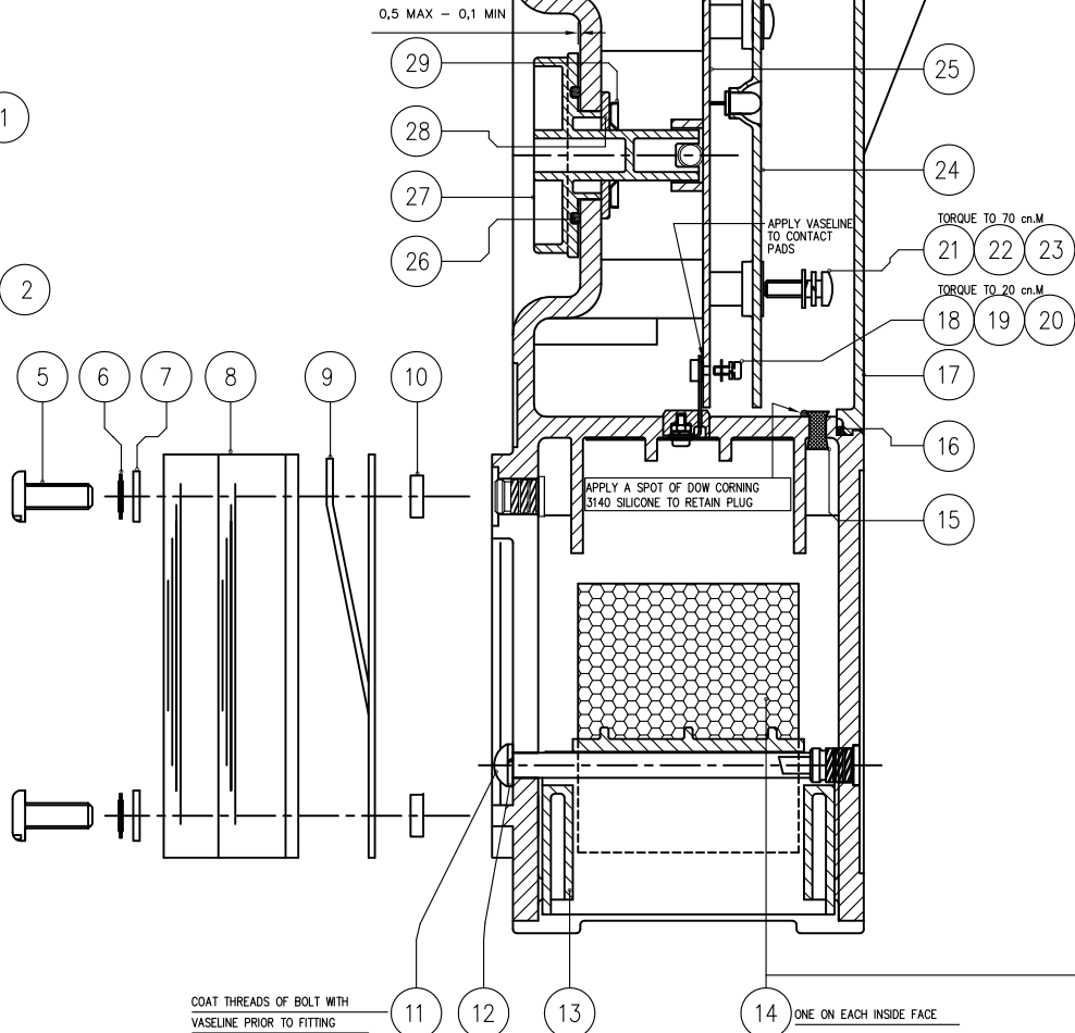
SWITCH ASSY 2:1 SHOWING LUBRICATION DETAILS
