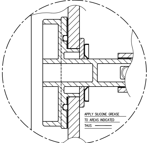
SWITCH ASSY 2:1 SHOWING LUBRICATION DETAILS
