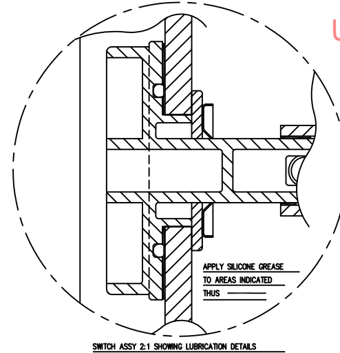
SWITCH ASSY 2:1 SHOWING LUBRICATION DETAILS
