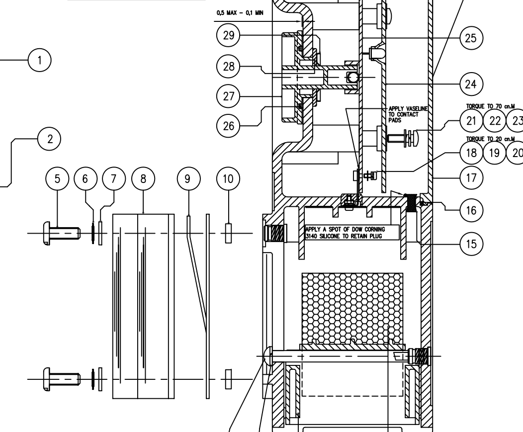
SWITCH ASSY 2:1 SHOWING LUBRICATION DETAILS
