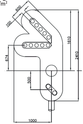
Type 16. 0086/009412 3 Aspect Colour Light Signal with Position 1+2+4+5 Junction Indicator and Position Light Signal Weight - 72kg Area - 2.582m 2
