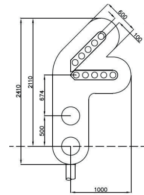
Type 57. 0086/009444 4 Aspect Colour Light Signal with Position 1+2+4 Junction Indicator Weight - 64kg Area - 1.266m 2
