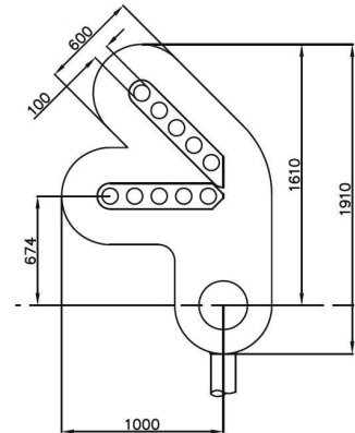
Type 5. 0086/009401 3 Aspect Colour Light Signal with Position 1+2 Junction Indicator Weight - 43kg Area - 1.527m 2
