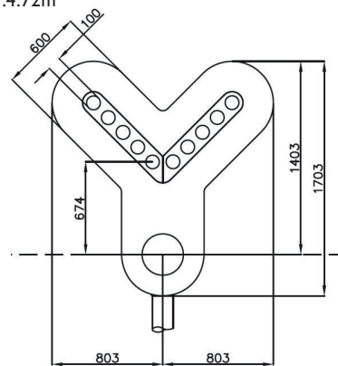
Type 4. 0086/009400 3 Aspect Colour Light Signal with Position 1+4 Junction Indicator Weight - 43kg Area - 1.472m 2
