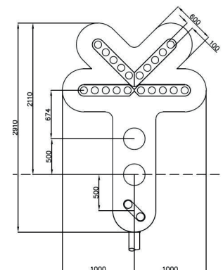
Type 65. 0086/009452 4 Aspect Colour Light Signal with Position 1+2+4+5 Junction Indicator and Position Light Signal Weight - 84kg Area - 2.882m 2
