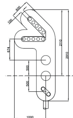
Type 63. 0086/009450 4 Aspect Colour Light Signal with Position 1+2 Junction Indicator and Position Light Signal Weight - 56kg Area - 2.127m 2
