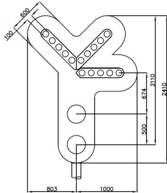
Type 58. 0086/009445 4 Aspect Colour Light Signal with Position 1+4+5 Junction Indicator Weight - 64kg Area - 2.241m 2
