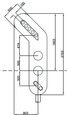
Type 60. 0086/009447 4 Aspect Colour Light Signal with Position 1 Junction Indicator and Position Light Signal Weight - 45kg Area - 1.080m 2
