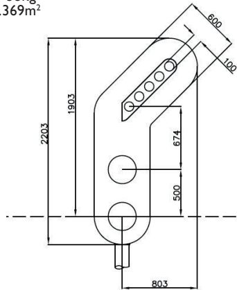
Type 52. 0086/009439 4 Aspect Colour Light Signal with Position 4 Junction Indicator Weight - 38kg Area - 1.369m 2
