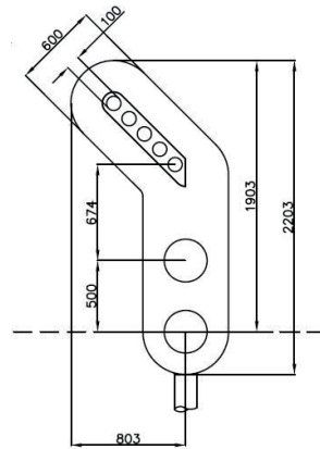
Type 53. 0086/009440 4 Aspect Colour Light Signal with Position 1+4 Junction Indicator Weight - 51kg Area - 1.772m 2
