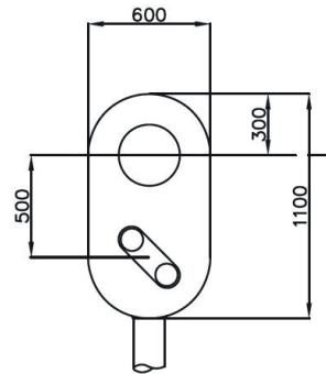
Type 10. 0086/009406 3 Aspect Colour Light Signal with Position Light Signal Weight - 19kg Area - 0.582m 2
