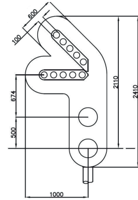
Type 56. 0086/009443 4 Aspect Colour Light Signal with Position 1+2+4+5 Junction Indicator Weight - 77kg Area - 1.108m 2
