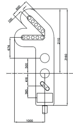
Type 81. 0086/009468 4 Aspect Colour Light Signal with Position 1+2 Junction Indicator, Position Light Signal and Miniature Alphanumeric Route Indicator (Stencil) Weight - 70kg Area - 2.315m 2
