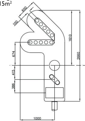
Type 32. 0086/009428 3 Aspect Colour Light Signal with Position 1+2 Junction Indicator and Position Light Signal and Miniature Alphanumeric Route Indicator (Stencil) Weight - 59kg Area - 2.015m 2
