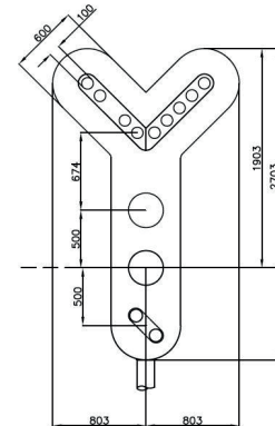
Type 62. 0086/009449 4 Aspect Colour Light Signal with Position 1+4 Junction Indicator and Position Light Signal Weight - 56kg Area - 2.072m 2
