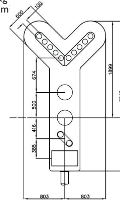
Type 80. 0086/009467 4 Aspect Colour Light Signal with Position 1+4 Junction Indicator, Position Light Signal and Miniature Alphanumeric Route Indicator (Stencil) Weight - 70kg Area - 2.260m 2
