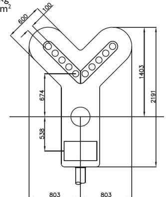
Type 24. 0086/009420 3 Aspect Colour Light Signal with Position 4+5 Junction Indicator and Miniature Alphanumeric Route Indicator (Stencil) Weight - 54kg Area - 1.857m 2
