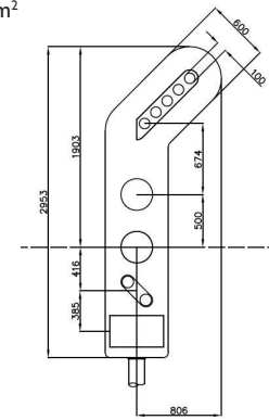
Type 81. 0086/009468 4 Aspect Colour Light Signal with Position 1+2 Junction Indicator, Position Light Signal and Miniature Alphanumeric Route Indicator (Stencil) Weight - 70kg Area - 2.315m 2
