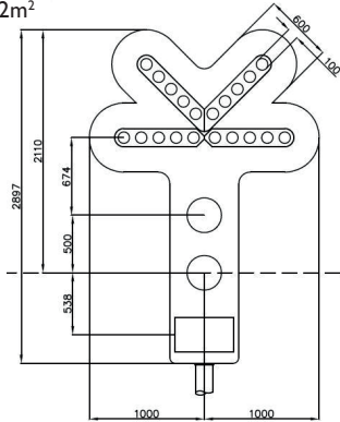
Type 76. 0086/009463 4 Aspect Colour Light Signal with Position 1+4+5 Junction Indicator and Miniature Alphanumeric Route Indicator (Stencil) Weight - 76kg Area - 2.571m 2
