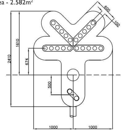
Type 16. 0086/009412 3 Aspect Colour Light Signal with Position 1+2+4+5 Junction Indicator and Position Light Signal Weight - 72kg Area - 2.582m 2
