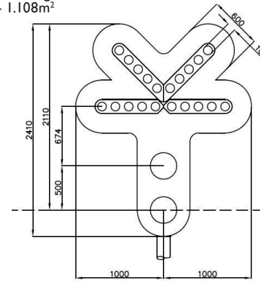
Type 56. 0086/009443 4 Aspect Colour Light Signal with Position 1+2+4+5 Junction Indicator Weight - 77kg Area - 1.108m 2
