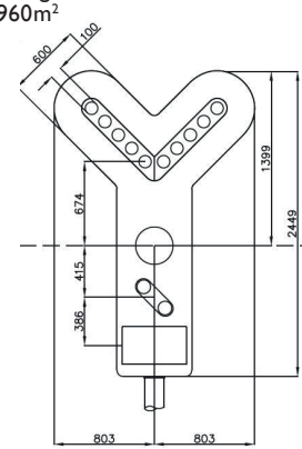
Type 31. 0086/009427 3 Aspect Colour Light Signal with Position 1+4 Junction Indicator and Position Light Signal and Miniature Alphanumeric Route Indicator (Stencil) Weight - 59kg Area - 1.960m 2
