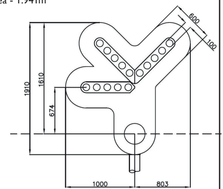
Type 8. 0086/009404 3 Aspect Colour Light Signal with Position 1+2+4 Junction Indicator Weight - 56kg Area - 1.941m 2
