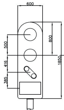
Type 77. 0086/009464 4 Aspect Colour Light Signal with Position Light Signal and Miniature Alphanumeric Route Indicator (Stencil) Weight - 39kg Area - 1.070m 2
