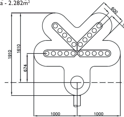
Type 7. 0086/009403 3 Aspect Colour Light Signal with Position 1+2+4+5 Junction Indicator Weight - 69kg Area - 2.282m 2
