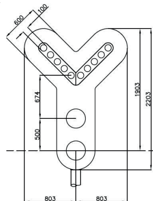
Type 53. 0086/009440 4 Aspect Colour Light Signal with Position 1+4 Junction Indicator Weight - 51kg Area - 1.772m 2
