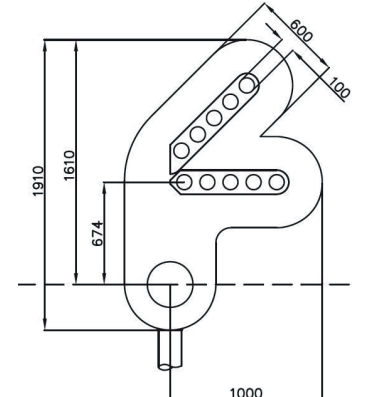
Type 8. 0086/009404 3 Aspect Colour Light Signal with Position 1+2+4 Junction Indicator Weight - 56kg Area - 1.941m 2
