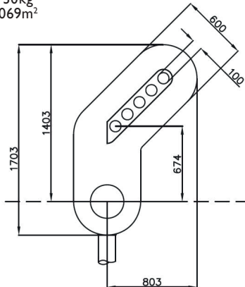
Type 3. 0086/009399 3 Aspect Colour Light Signal with Position 4 Junction Indicator Weight - 30kg Area - 1.069m 2
