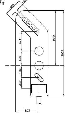
Type 80. 0086/009467 4 Aspect Colour Light Signal with Position 1+4 Junction Indicator, Position Light Signal and Miniature Alphanumeric Route Indicator (Stencil) Weight - 70kg Area - 2.260m 2
