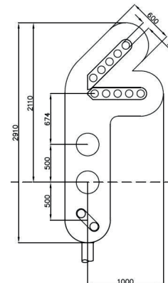
Type 64. 0086/009451 4 Aspect Colour Light Signal with Position 4+5 Junction Indicator and Position Light Signal Weight - 56kg Area - 2.127m 2
